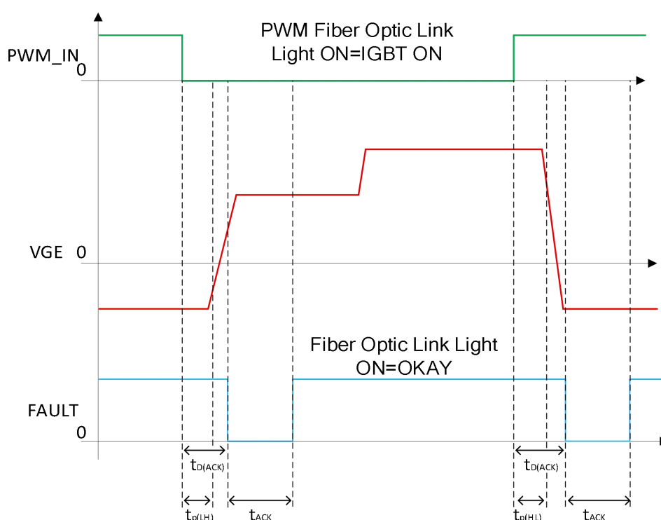
Fig.12a Normal condition
