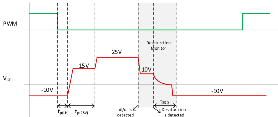
Fig.12c di/dt desaturation occurs during a fault condition.
