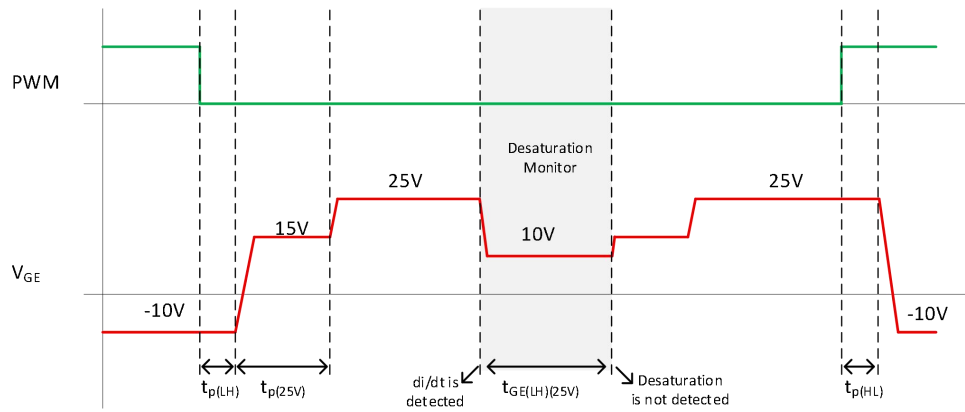
Fig.12b di/dt No desaturation occurred during the fault condition.
