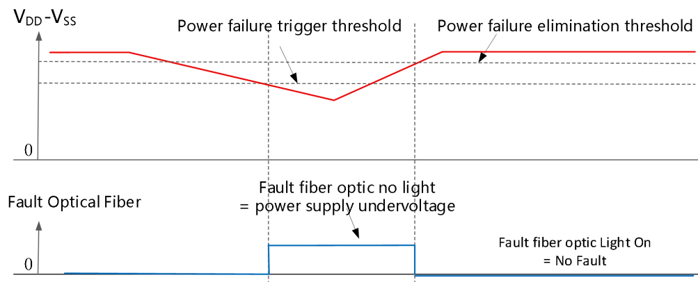
Fig.8 Undervoltage protection logic
