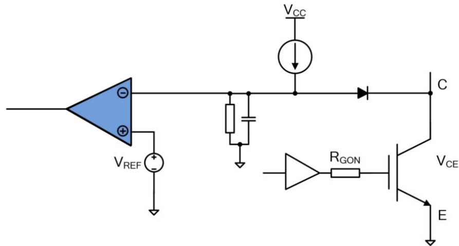
Fig.7 V_{CE} Short Circuit Detection Circuit
