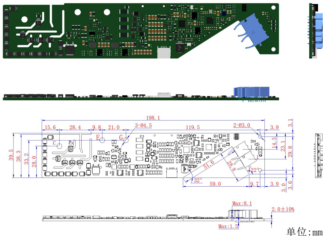
Fig.3 1FHD0440 3D and mechanical dimensions (unit: mm)
