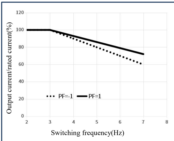
Fig.1 Output current versus switching frequency curve ( V_{DC}=1500 V, V_{AC} = 690 V RMS , f_{AC \text{ sine}} = 50 Hz, T_{inlet} = 45^{\circ}\text{C} )
