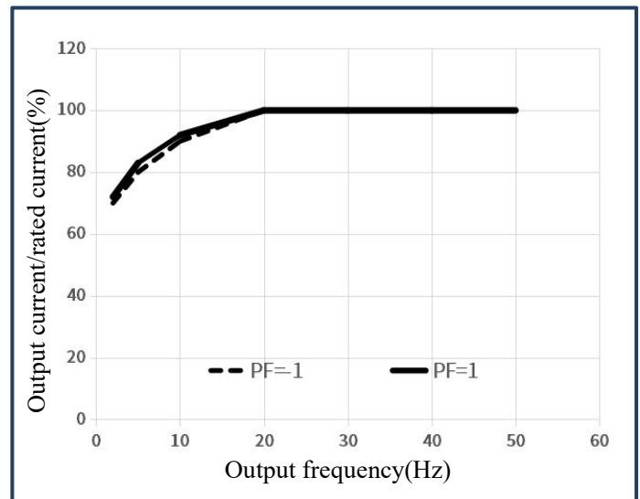
Fig.2 Output current versus output frequency curve ( V_{DC}=1500 V, V_{AC} = 690 V RMS , f_{SW} = 3 kHz, T_{inlet} = 45^{\circ}\text{C} )
