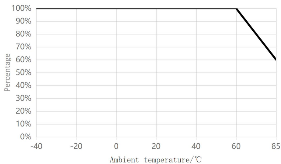
Fig.7 Derating curve
