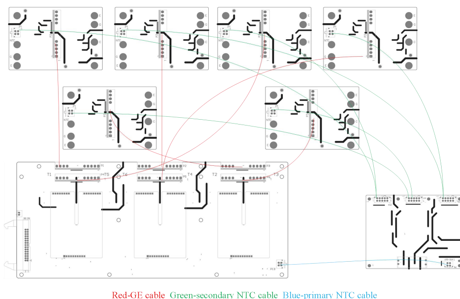
Fig.3 Connection schematic
