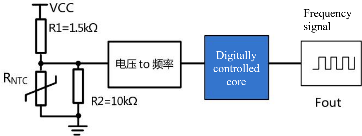
Fig.9 Temperature monitoring schematic
