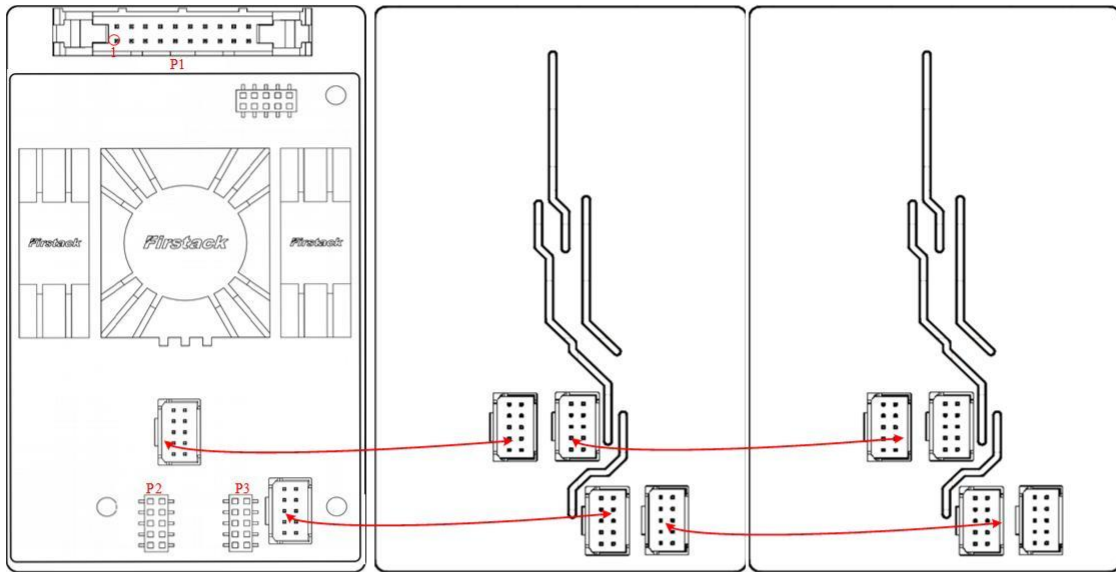
2FHD0620M17A1-Y0002+A1EDA1V-S0002 并联接线示意图
