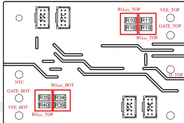
Fig.3 Connector interface designation
