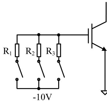
Fig.10 Multi-level turn-off schematic
