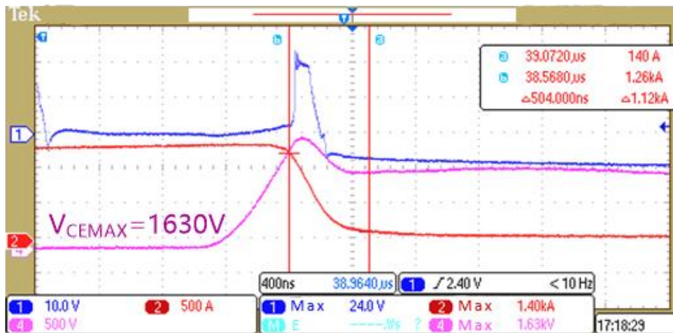
Fig.11a Without multi-level turn-off
